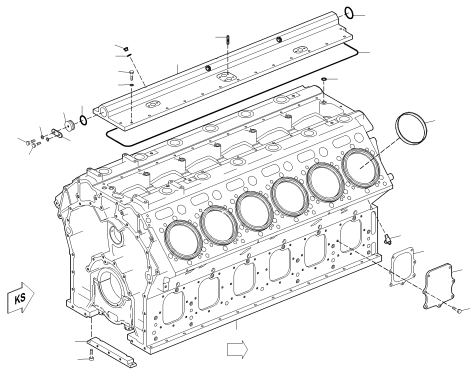
CRANKCASE UPC.06A01 2080
