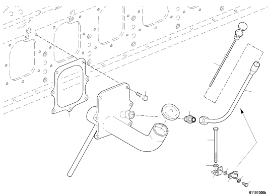
OIL FILLER NECK UPC.06G04 1432
